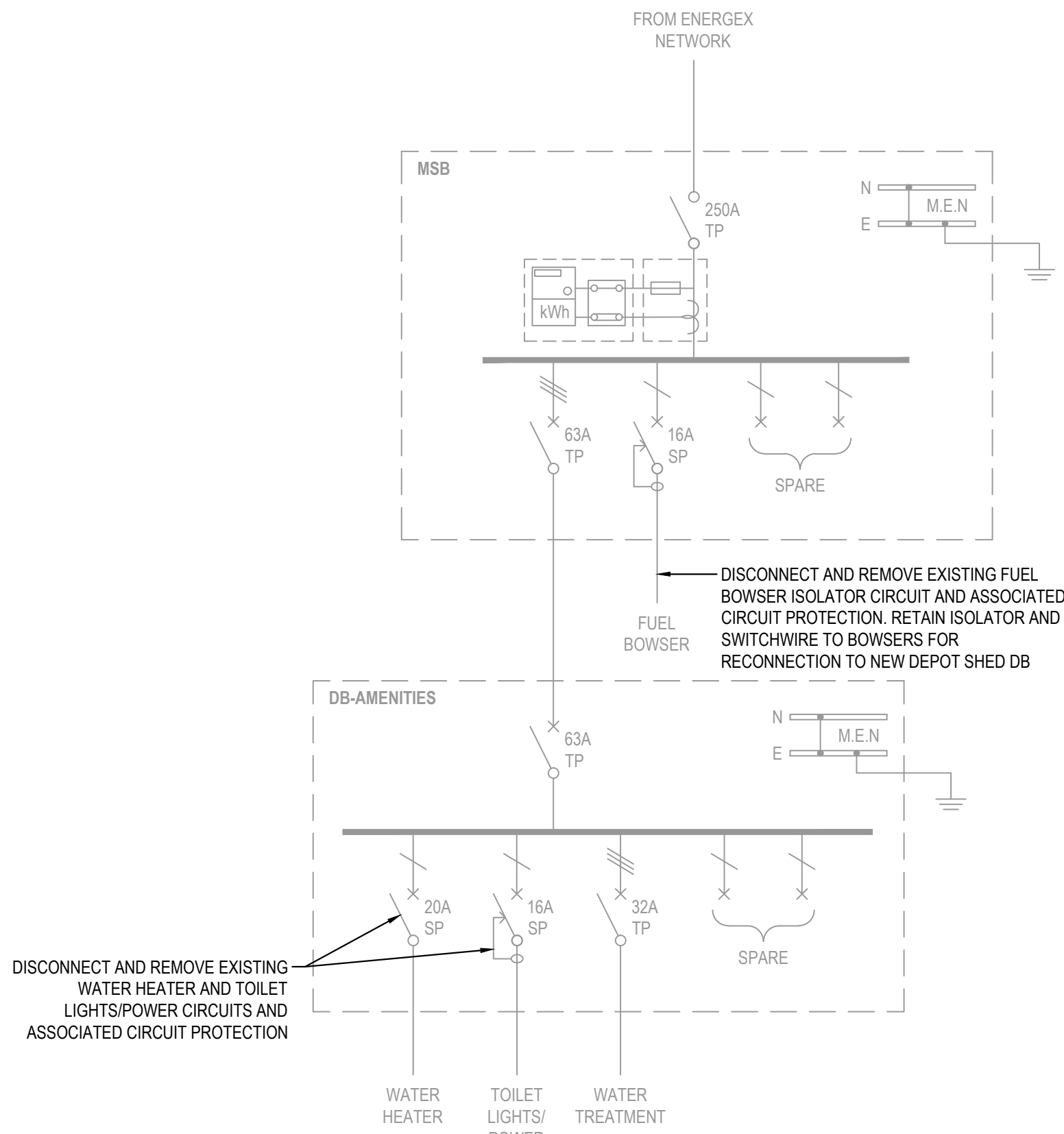
EXISTING SINGLE LINE DIAGRAM
