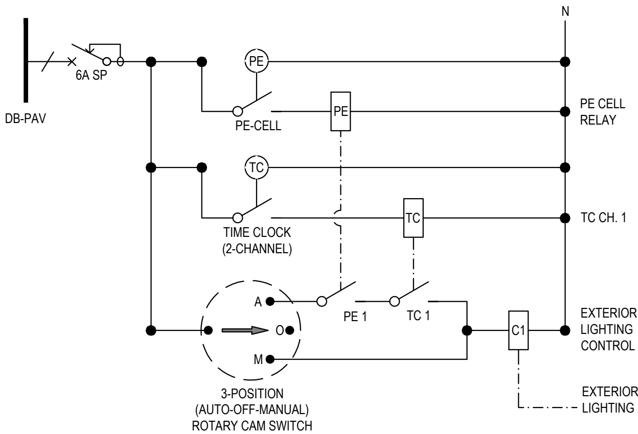
EXTERIOR LIGHTING CONTROL SCHEMATIC
